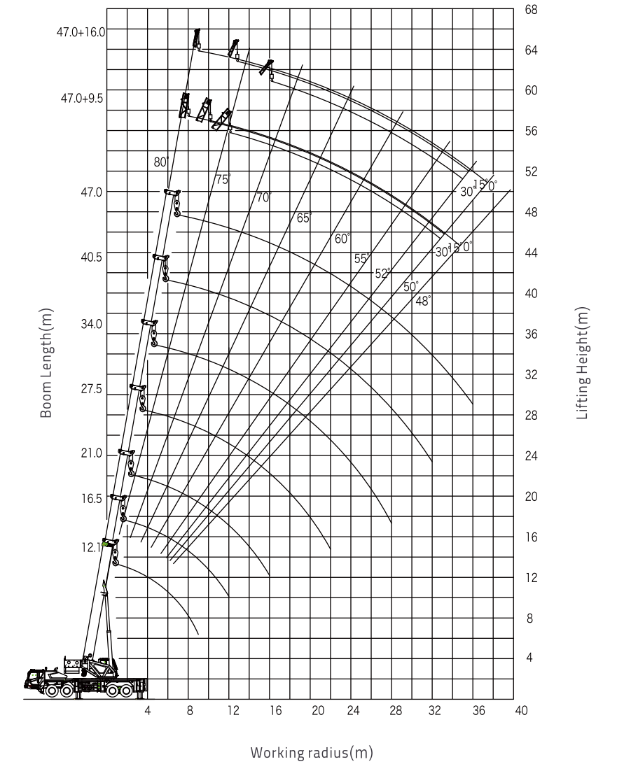
Lifting height curve
